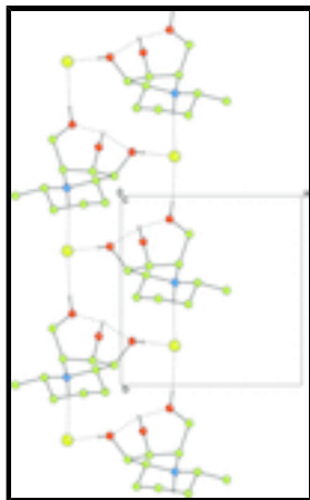
Fig. 3. 1 forms hydrogen bonded double chains around around the twofold screw axis parallel to the b -axis (viewed down the c -axis). Hydrogen bonding interactions are shown as dotted lines and all hydrogen atoms not involved are omitted for clarity.
