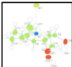
Fig. 2. The molecular structure of the title compound with displacement ellipsoids drawn at the 50% probability level. Hydrogen bonds are shown with a dotted lines.
